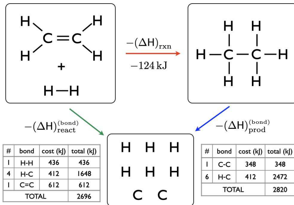
Figure 2.38: Calculation of reaction enthalpy for the hydrogenation of ethene (ethylenes), C_2H_4 .
