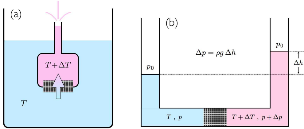
Figure 5.13: The fountain effect. In each case, a temperature gradient is maintained across a porous plug through which only superfluid can flow. This results in a pressure gradient which can result in a fountain or an elevated column in a U-tube.
