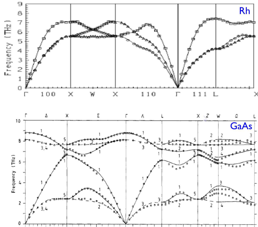
Figure 5.6: Upper panel: phonon spectrum in elemental rhodium (Rh) at T = 297 K measured by high precision inelastic neutron scattering (INS) by A. Eichler et al. , Phys. Rev. B 57 , 324 (1998). Note the three acoustic branches and no optical branches, corresponding to d = 3 and r = 1 . Lower panel: phonon spectrum in gallium arsenide (GaAs) at T = 12 K, comparing theoretical lattice-dynamical calculations with INS results of D. Strauch and B. Dorner, J. Phys.: Condens. Matter 2 , 1457 (1990). Note the three acoustic branches and three optical branches, corresponding to d = 3 and r = 2 . The Greek letters along the x -axis indicate points of high symmetry in the Brillouin zone.
