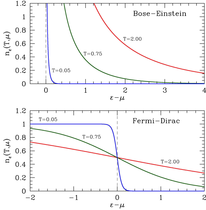
Figure 5.1: Occupation number versus \epsilon - \mu for Bose and Fermi distributions.
