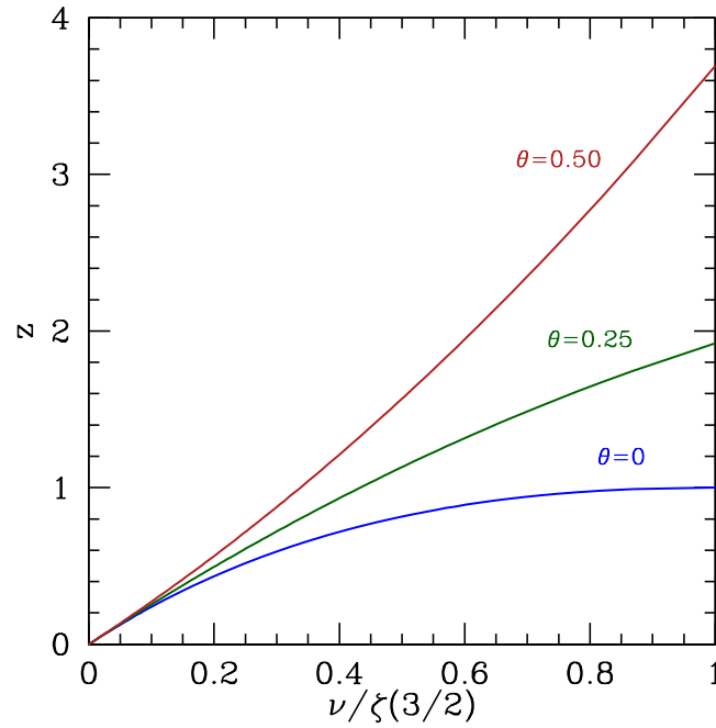
Figure 5.10: Fugacity z versus dimensionless density \nu = n\lambda_T^3 for the mean field interacting Bose gas.
