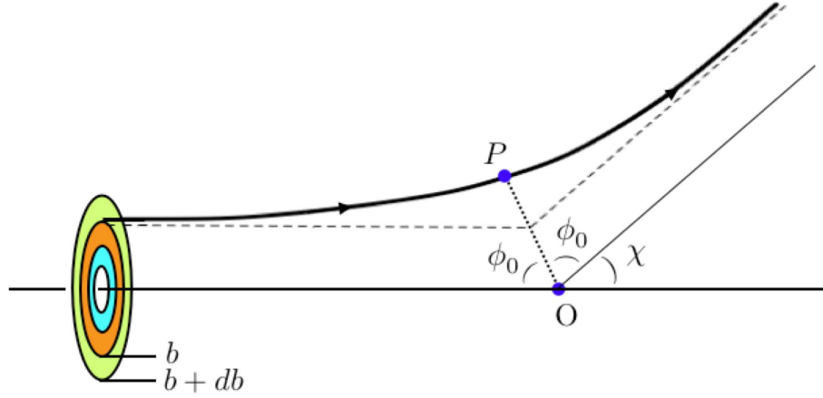
Figure 8.6: Scattering in the CM frame. O is the force center and P is the point of periastris. The impact parameter is b , and \chi is the scattering angle. \phi_0 is the angle through which the relative coordinate moves between periastris and infinity.
