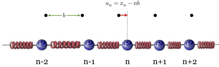
Figure 5.4: A linear chain of masses and springs. The black circles represent the equilibrium positions of the masses. The displacement of mass n relative to its equilibrium value is u_n .
