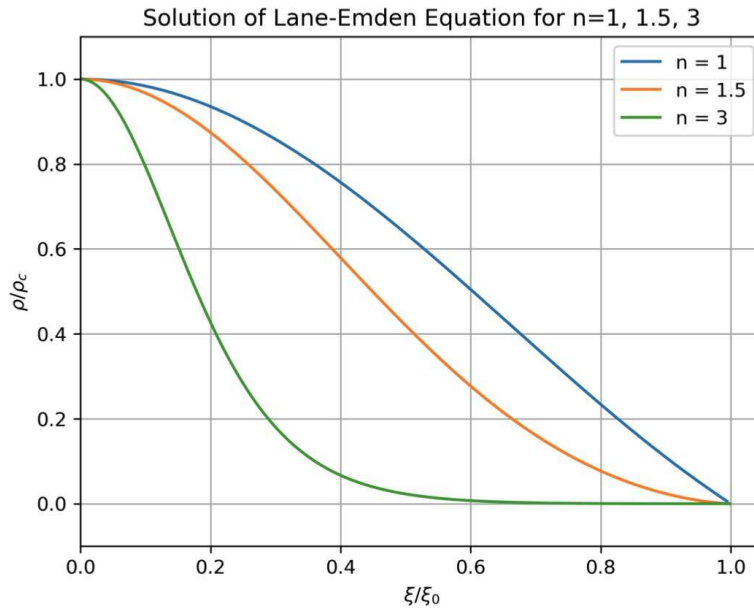
Figure 5.21: Solutions to the Lane-Emden equation for n = 1 , n = \frac{3}{2} , and n = 3 .
