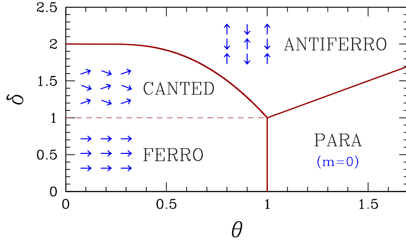
Figure 7.27: Mean field phase diagram for the model of eqn. 7.343 for the case \kappa = 1 .
